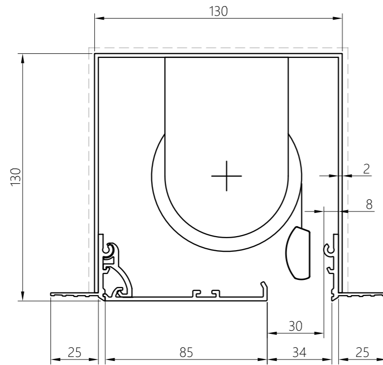
HEAD BOX C130x130SS
