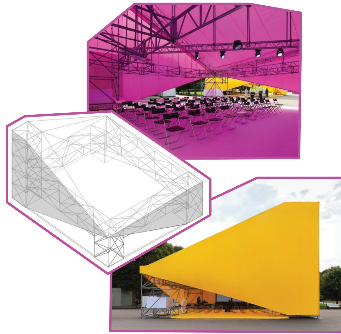
Reimagining a tent-like structure. Notable "post and beam" scaffolding achieving wide span. Expensive.
