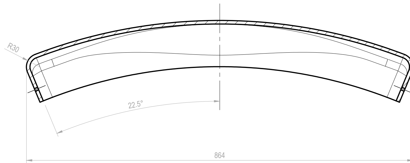
B-B (1:5)
