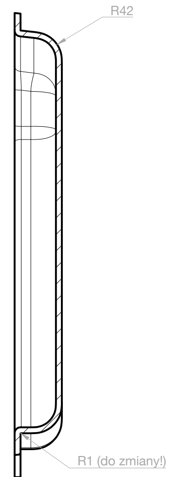
B-B (1:5)
