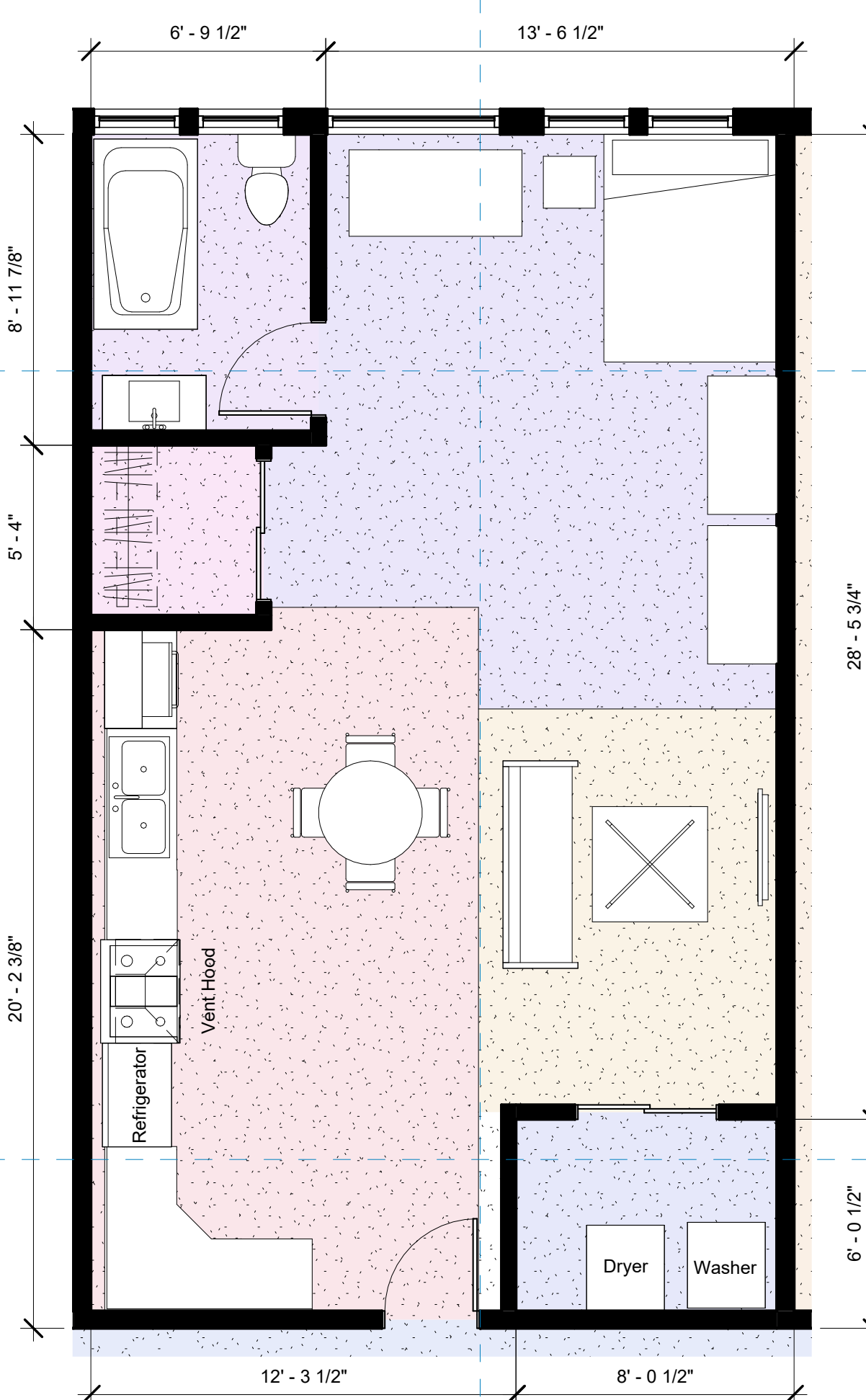
1 BLDG1 Floor 1 - Callout 2 1/4" = 1'-0"
