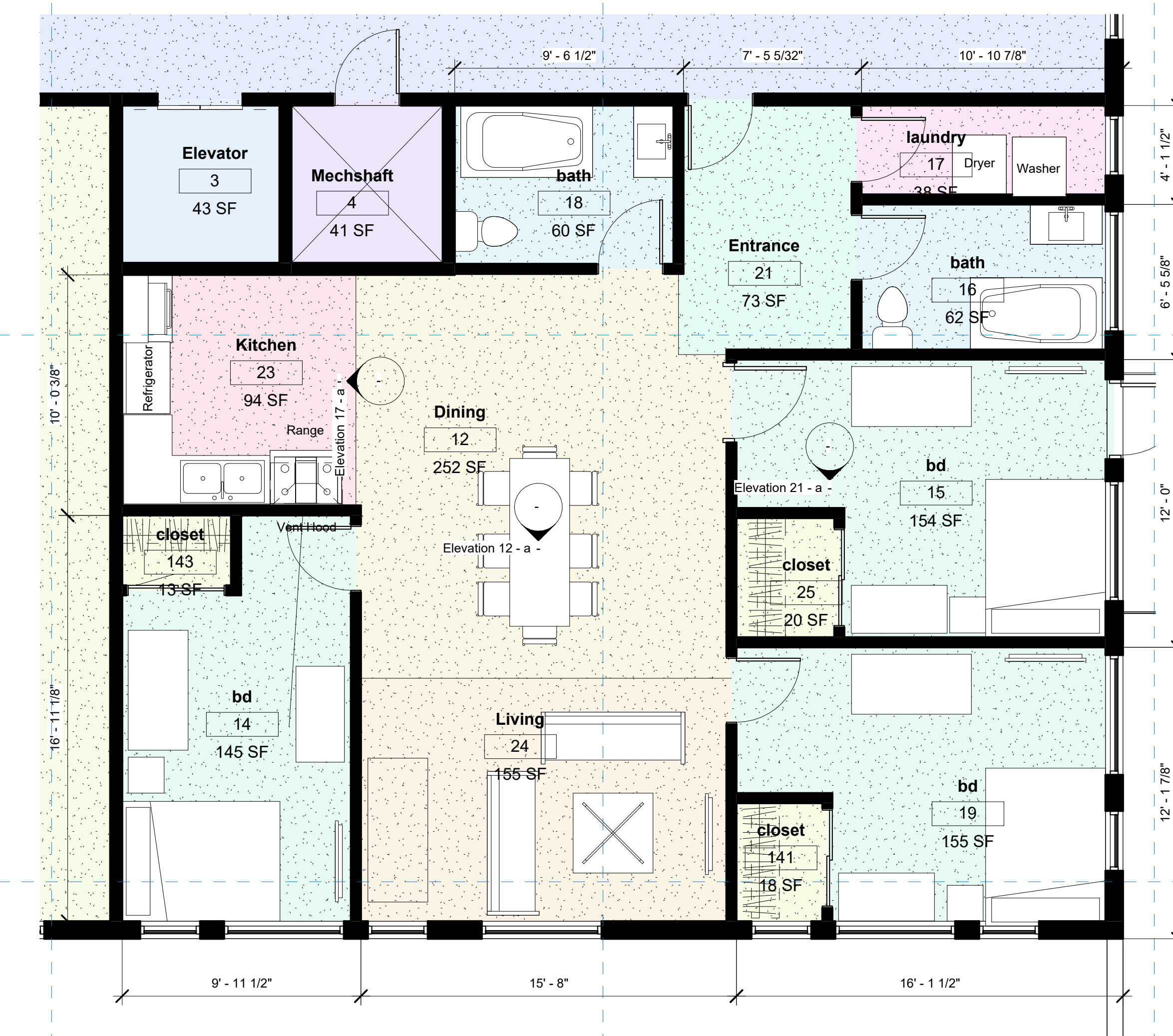
1 BLDG1 Floor 1 - Callout 1 1/4" = 1'-0"
