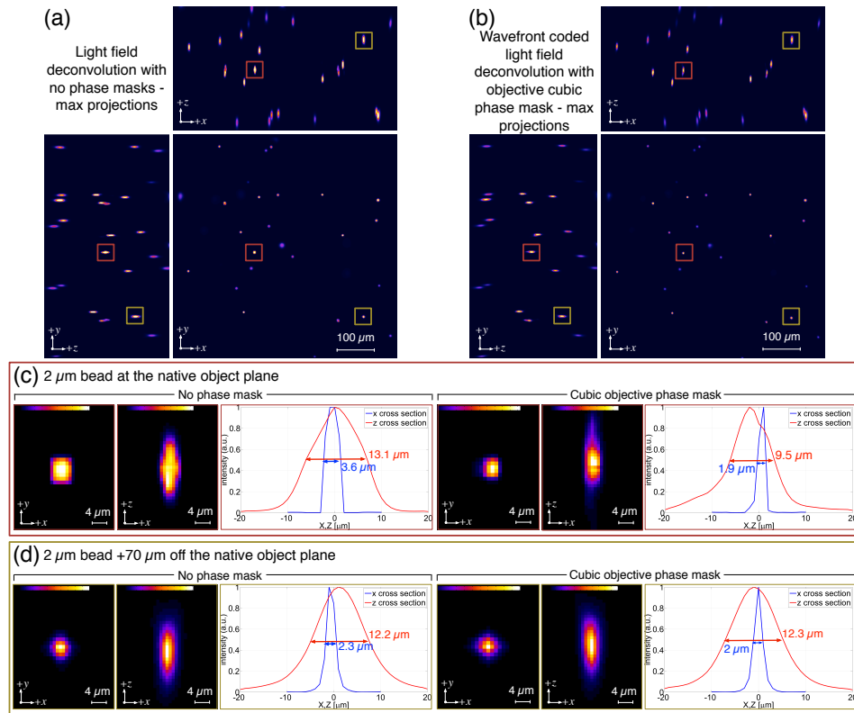
Fig. 6. Volumetric imaging of 2 μm fluorescent beads embedded in agarose, with and without an objective cubic phase mask. (a) Max projections through the volume with no phase mask. (b) Max projections through the volume with the cubic phase mask. (c) Reconstructed bead on the native object plane (red boxes in (a) and (b)) and the corresponding X and Z intensity profiles showing the FWHM for each case. The cubic mask significantly improves both lateral resolution and axial resolution. (d) Reconstructed bead +70 μm off the native object plane (yellow boxes in (a) and (b)). The phase mask improves the lateral resolution slightly but the axial resolution remains the same as the no phase mask case.
